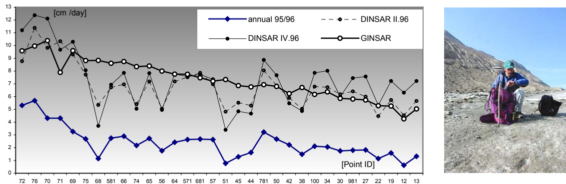
Fig. 5. Interferometric velocities (cm/day) versus average annual velocities 1995/96 on Hintereisferner Glacier.
