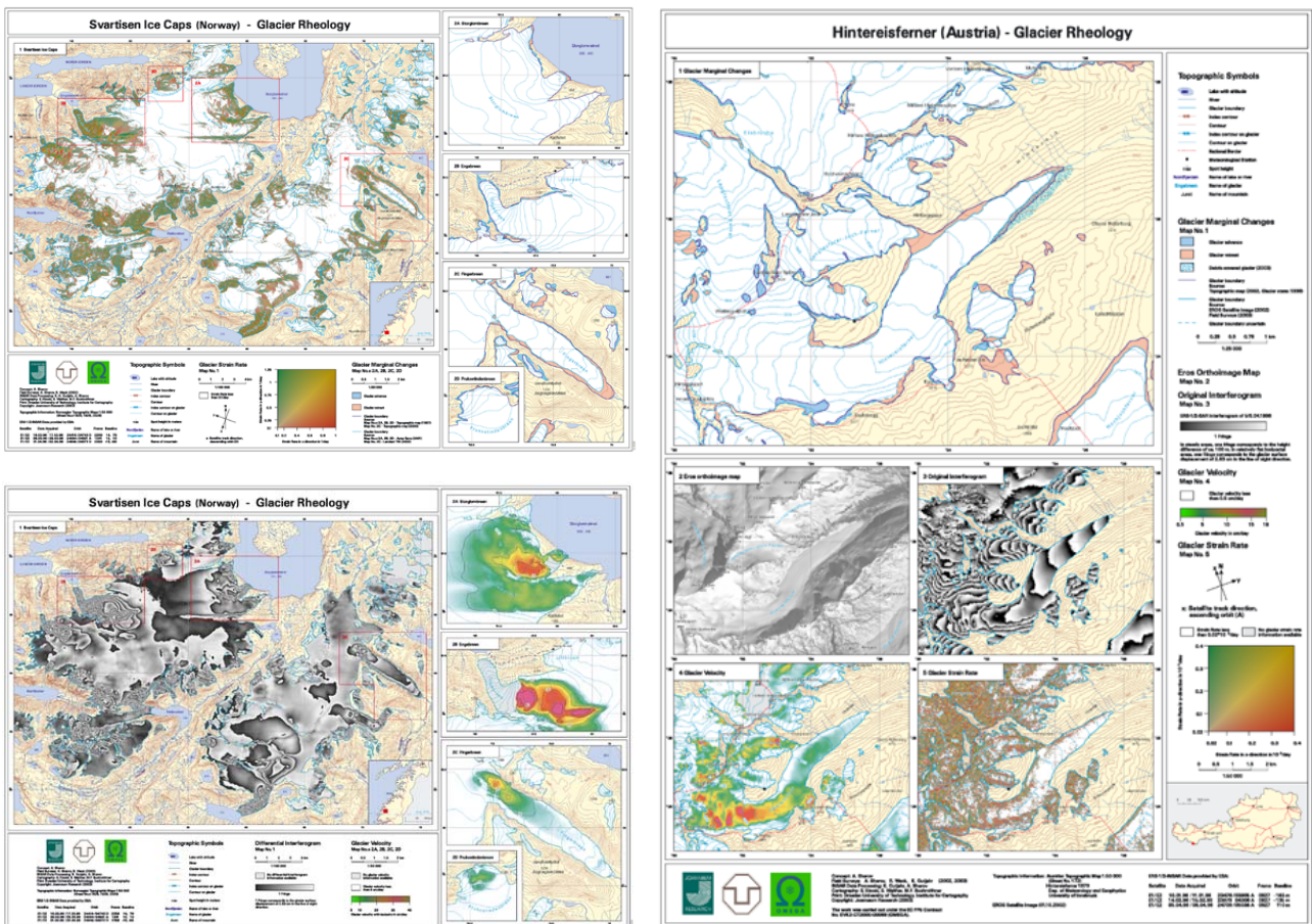
Fig. 4. Satellite rheological image maps of Svartisen Ice Caps, Northern Norway (on the left) and Hintereisferner Glacier, Oetztal Alps (on the right).
