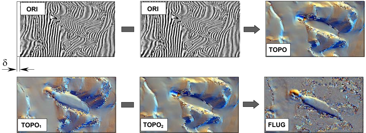
Fig. 1. Underlying concept of the GINSAR method
