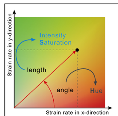
Fig. 3. Representation of the glacier strain rate using IHS-colour system
